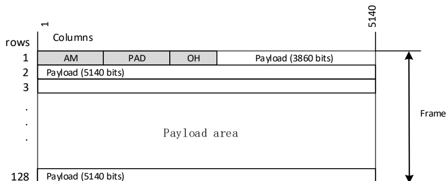
Figure 6. FlexO frame structure.
