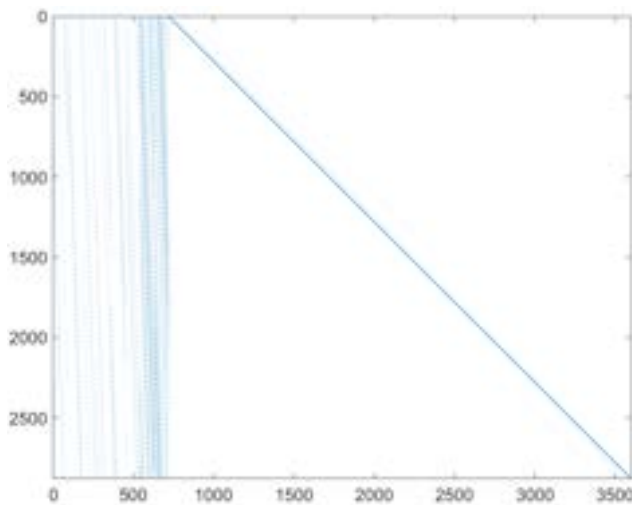
Figure 25. H matrix (IRA form) of code ( n=3600 , k=720 , rate 0.2)
